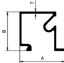
GLAZING CLIP
