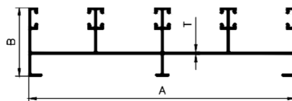
4 TRACK TOP
