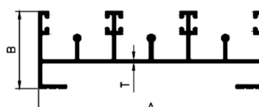
3 TRACK BOTTOM
