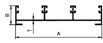
3 TRACK TOP
