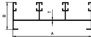
3 TRACK TOP
