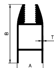
GLASS BOTTOM
