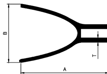
LOUVERS BRACKET
