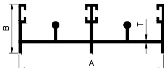
2 TRACK BOTTOM
