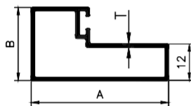
L PIPE
