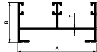
2 TRACK TOP
