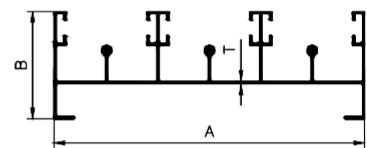
TRACK BOTTOM
