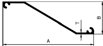
LOUVERS PLATE
