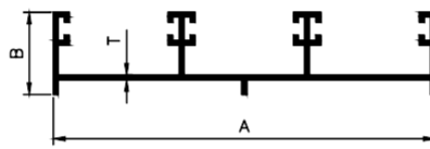
3 TRACK TOP
