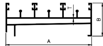
3 TRACK BOTTOM
