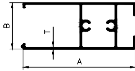
BEARING BOTTOM
